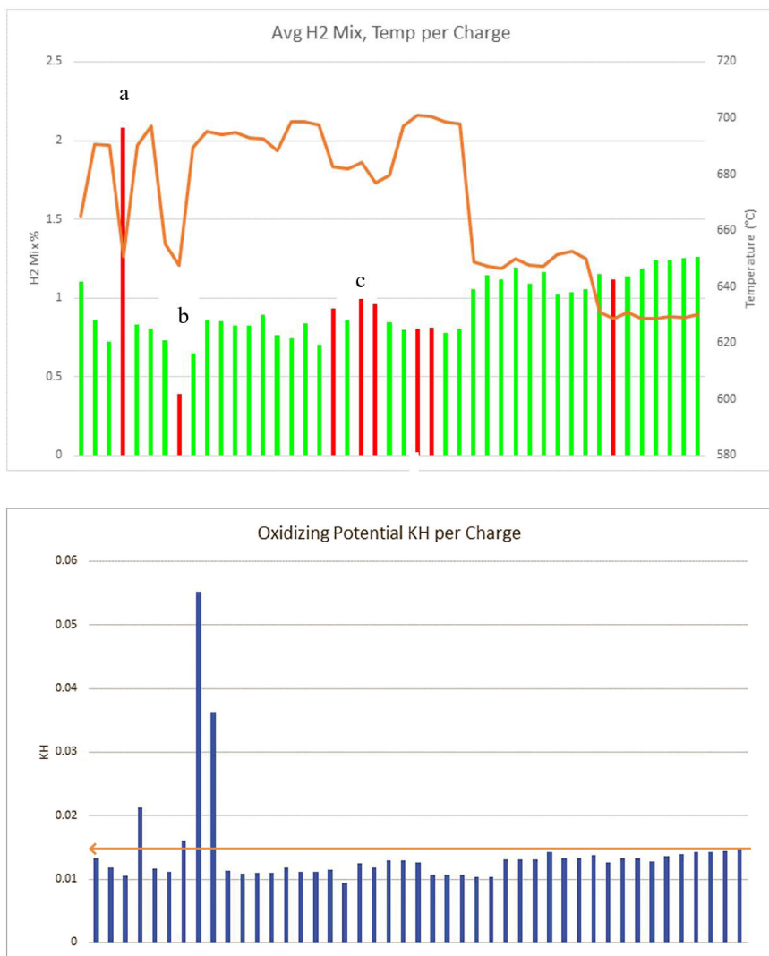
Figure 5: Example of atmosphere compositions for several charges at different annealing temperature
