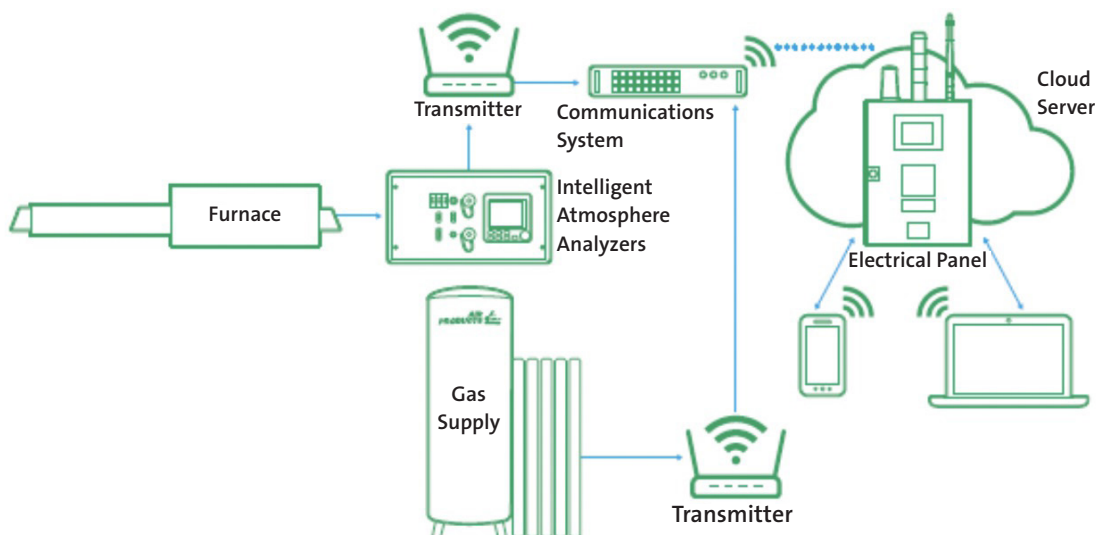
Figure 3: Set-up of the Cloud based Advisor System
