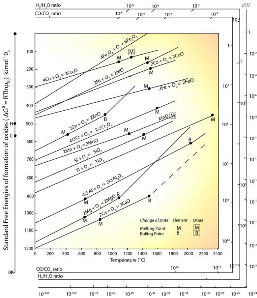
Figure 4: Ellingham-Richardson Diagram [3]
